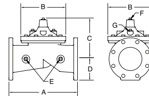
Reduced Port Body
