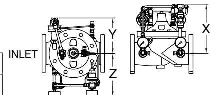
Globe Pilot System Dimensions
