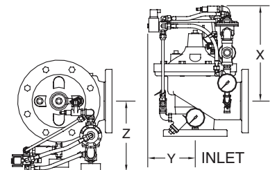
Angle Pilot System Dimensions
